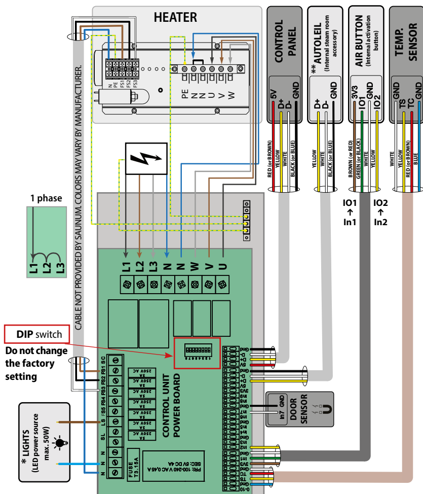
Figure 13 Connecting to the control unit.
